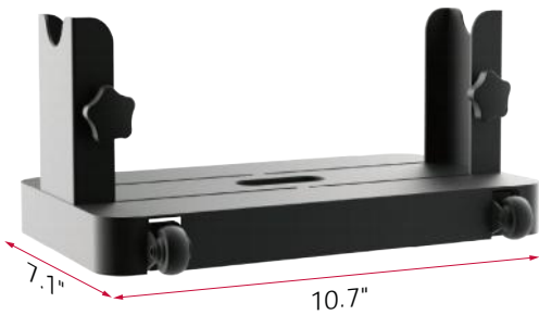
Folding floor stand 2 wheels (Standard)
